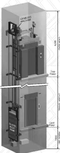
(SECTION : A-A) LIFT WELL
