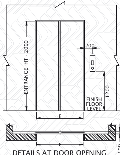
DETAILS AT DOOR OPENING
