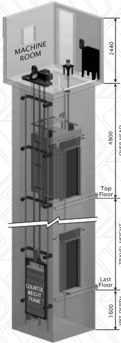
(SECTION : X-X) LIFT WELL
