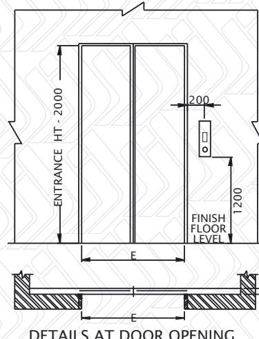
DETAILS AT DOOR OPENING
