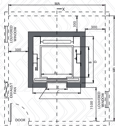
LIFT SHAFT, CAR, C.W. & MACHINE ROOM PLAN
