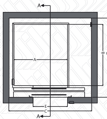
LIFT SHAFT, CAR, & C.W. PLAN
