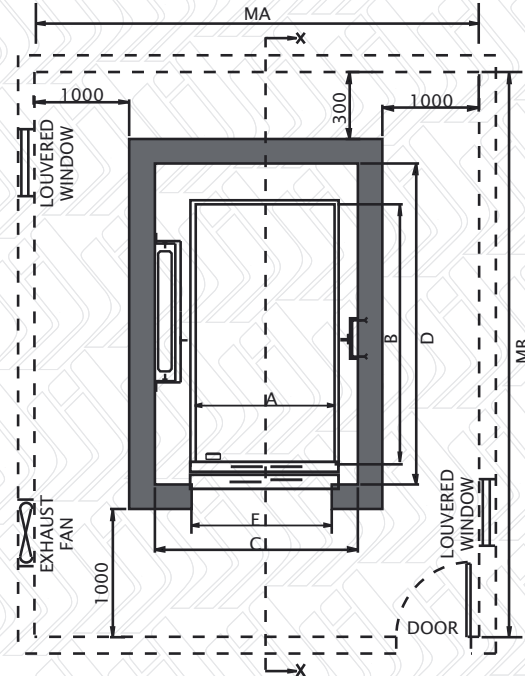
LIFT SHAFT, CAR, C.W. & MACHINE ROOM PLAN
