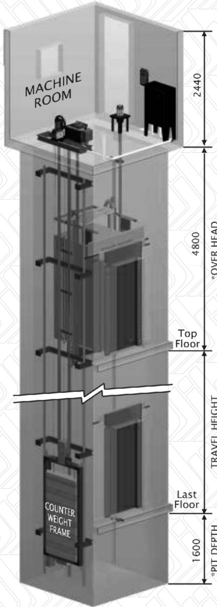
( SECTION : X-X ) LIFT WELL
